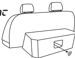
OPTION 2 Bassreflex port front Sound transmission directly into the trunk
